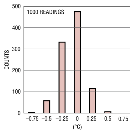
T_{INT} Noise
