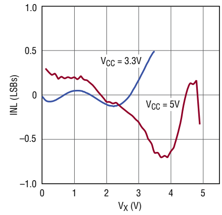
Single-Ended INL
