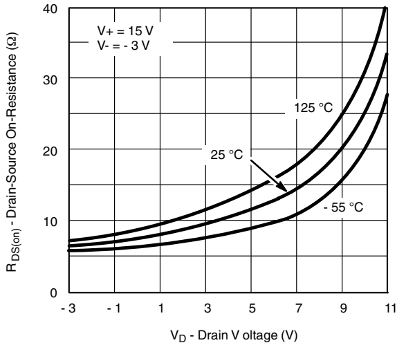
DG641, DG643 R_{\text{DS(on)}} vs. Drain Voltage
