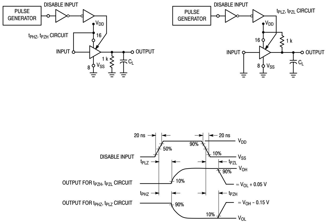
Figure 2. 3-State AC Test Circuit and Waveforms (t PLZ , t PHZ , t PZH , t PZL )
