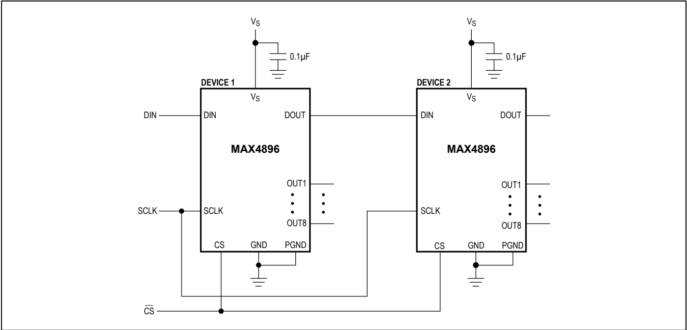
Figure 3. Daisy-Chain Configuration
