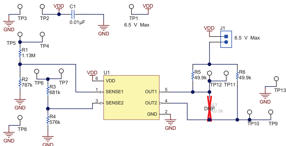
Figure 5. TPS3780EVM-154 Schematic
