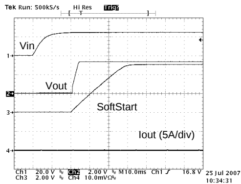
Figure 5. Start-Up Response: No Load
