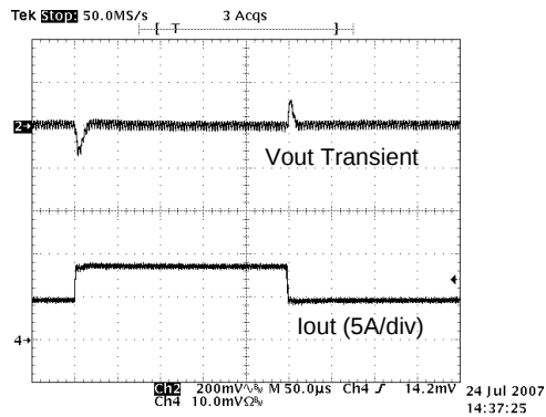
Figure 3. Load Step Response: 4->8A
