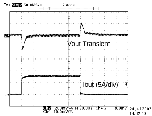
Figure 4. Load Step Response: 0->8A
