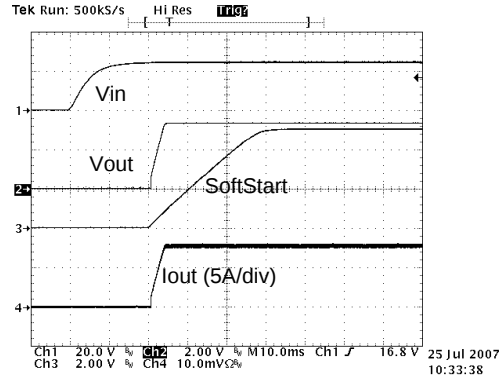
Figure 6. Start-Up Response: 8.0A Load
