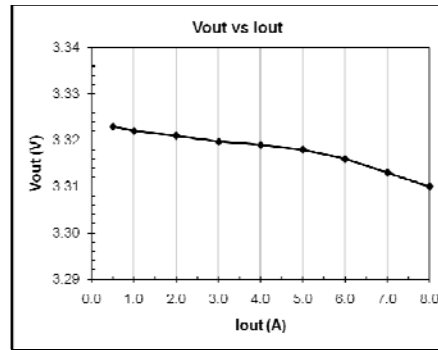
Figure 2. Load Regulation
