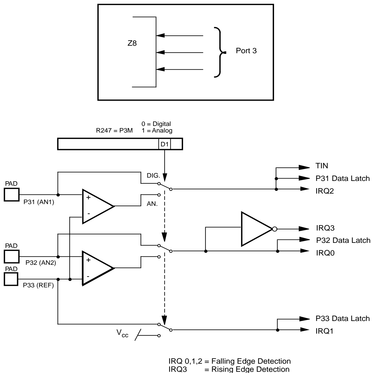
Figure 9. Port 3 Configuration
