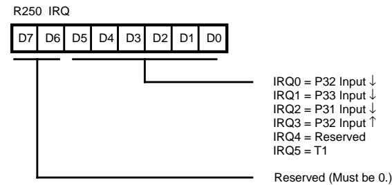
Figure 25. Interrupt Request Register (FA H : Read/Write)
