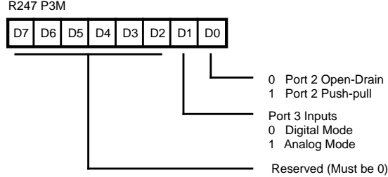
Figure 22. Port 3 Mode Register (F7 H : Write Only)
