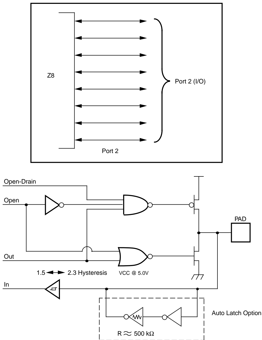
Figure 8. Port 2 Configuration
