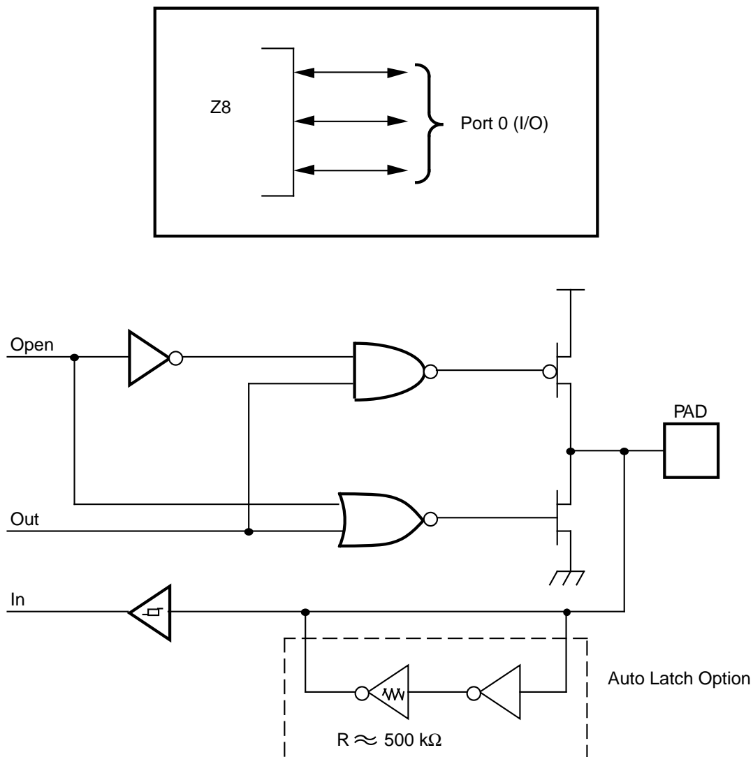
Figure 7. Port 0 Configuration
