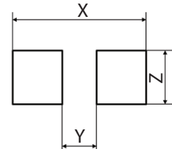
SUGGESTED LAND PATTERN
