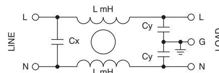
CIRCUIT DIAGRAM
