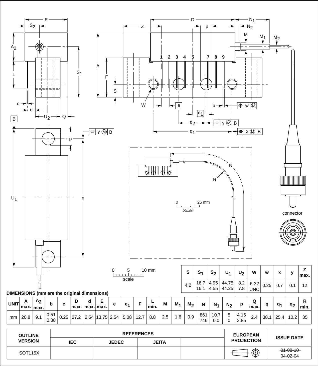
Fig 3. Package outline SOT115X
