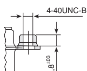
E Clinch nut 4-40UNC
