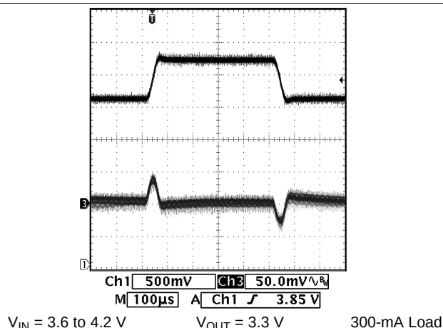
Figure 6. Line Transient (LDO2)
