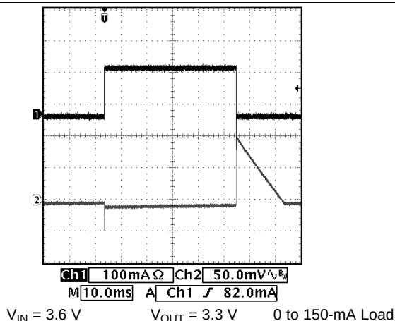
Figure 4. Load Transient (LDO2)
