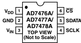
6-Lead SC70
