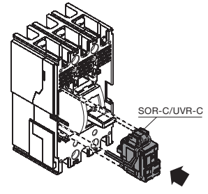
Three-pole circuit breaker
