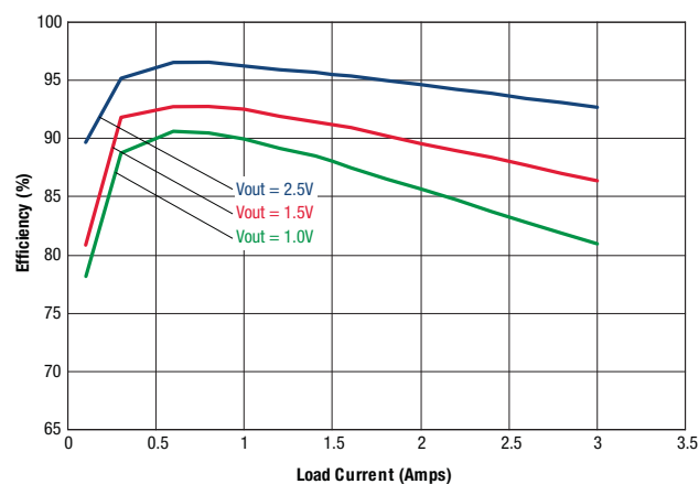
Efficiency vs. Line Voltage and Load Current @ +25°C ( V_{IN} = 3.3V )
