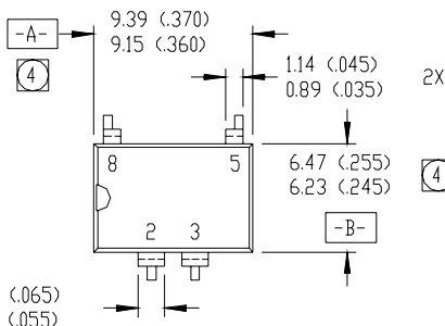
PVI5050N/PVI5080N
