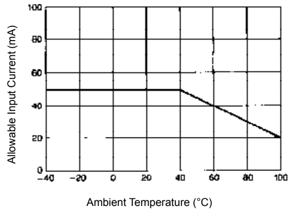
Figure 4. Input Current Derating
