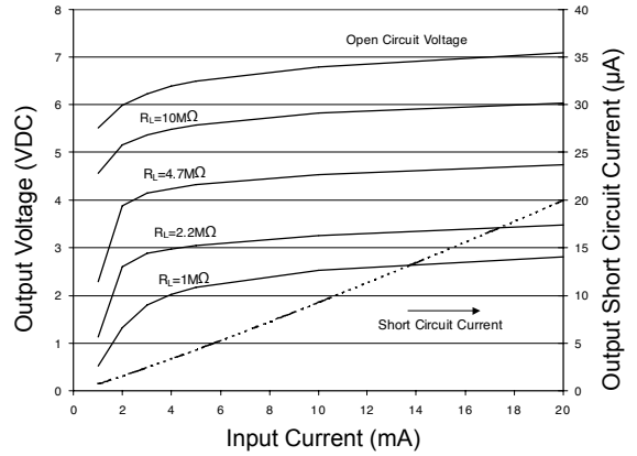
Figure 2. PVI5080N Typical Output Characteristics
