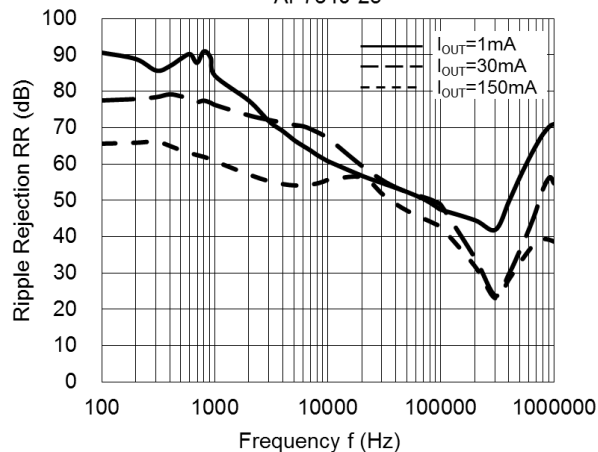
Ripple Rejection vs. Frequency AP7340-25
