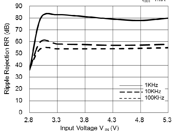
Ripple Rejection vs. Input Bias Voltage AP7340-28 I_{OUT}=1mA
