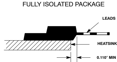
Figure 11. Mounting Position
