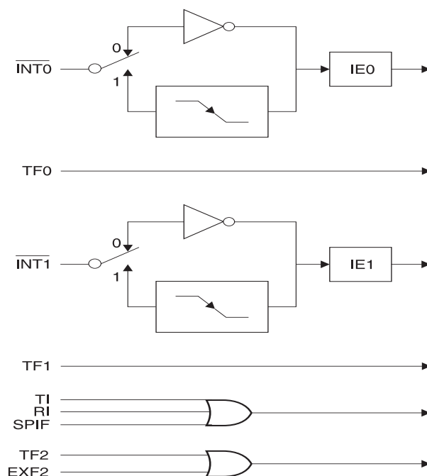
Figure 10. Interrupt Sources
