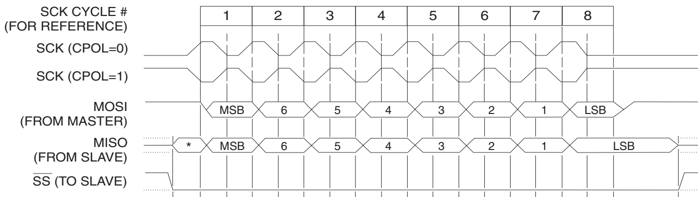
Figure 9. SPI Transfer Format with CPHA = 1
