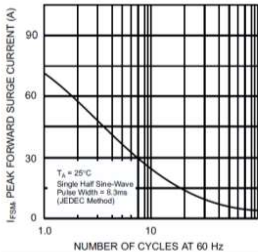
Figure 3 Maximum Peak Forward Surge Current (Per Leg)
