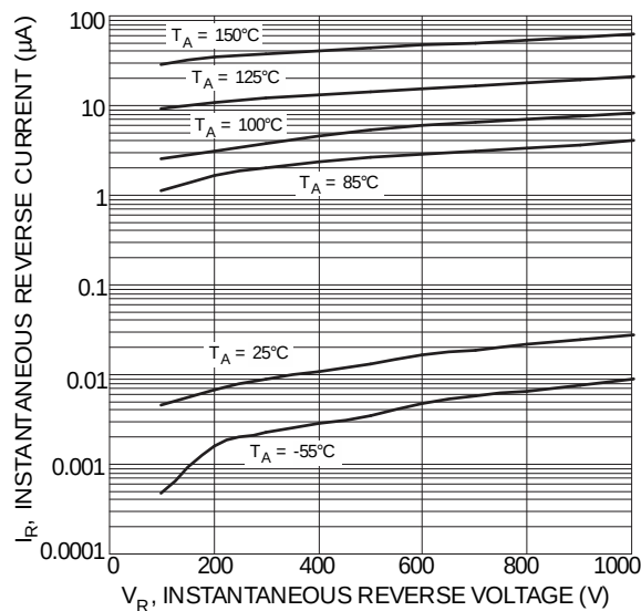
Figure 5 Typical Reverse Characteristics (Per Leg)
