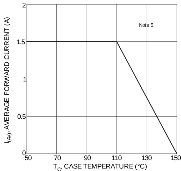
Figure 1 Output Current Derating Curve
