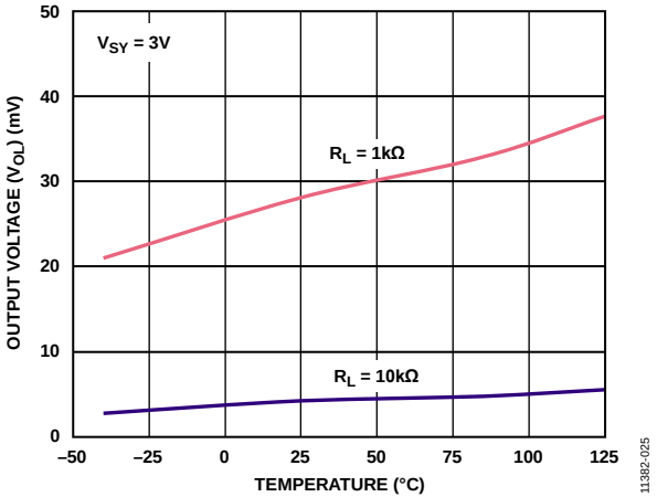
Figure 26. Output Voltage ( V_{OU} ) vs. Temperature
