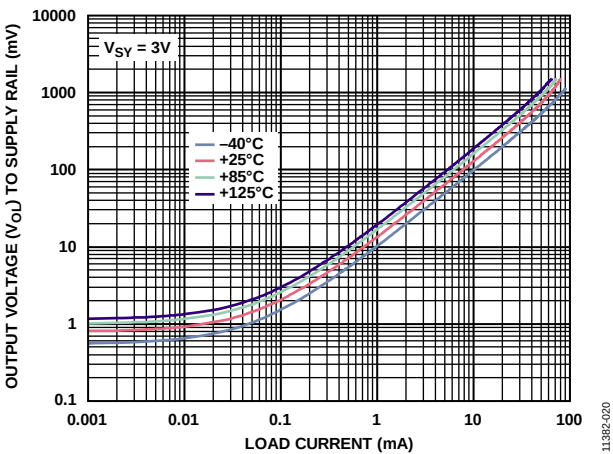
Figure 24. Output Voltage ( V_{OU} ) to Supply Rail vs. Load Current
