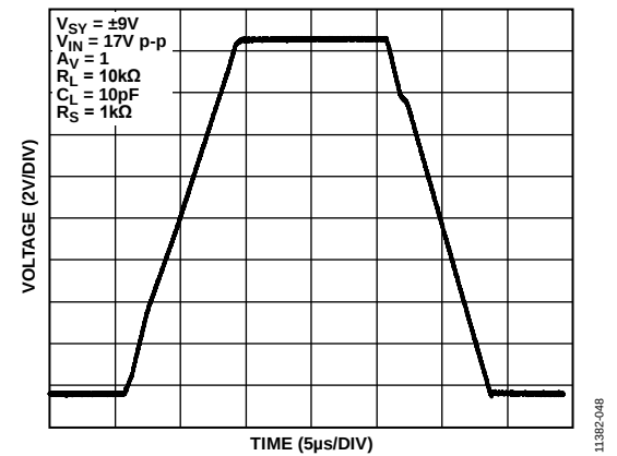
Figure 47. Large Signal Transient Response
