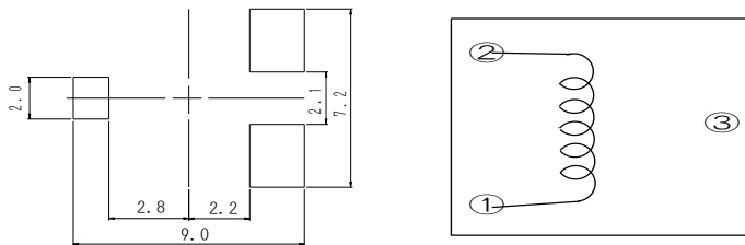
Land pattern and Schematics - [mm]
