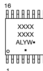
TSSOP-16 DT SUFFIX CASE 948F
