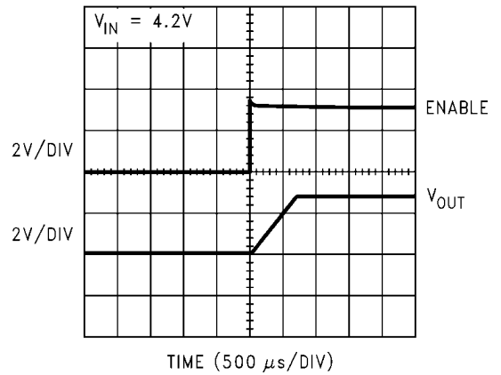
T_{\text{SLEEP}} @ MODE = 0V, C_{\text{OUT}} = 4.7\mu\text{F} , I_{\text{L}} = 1\text{mA}
