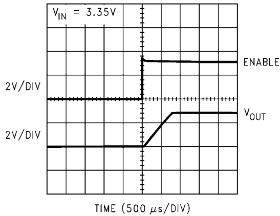
T_{\text{SLEEP}} @ MODE = 0V, C_{\text{OUT}} = 4.7\mu\text{F} , I_{\text{L}} = 1\text{mA}
