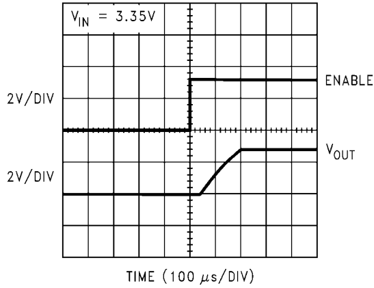
T_{\text{SLEEP}} @ MODE = 0V, C_{\text{OUT}} = 1\mu\text{F} , I_{\text{L}} = 1\text{mA}
