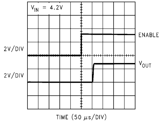
T_{\text{ON}} @ MODE = 1.8V, C_{\text{OUT}} = 1\mu\text{F} , I_{\text{L}} = 150\text{mA}
