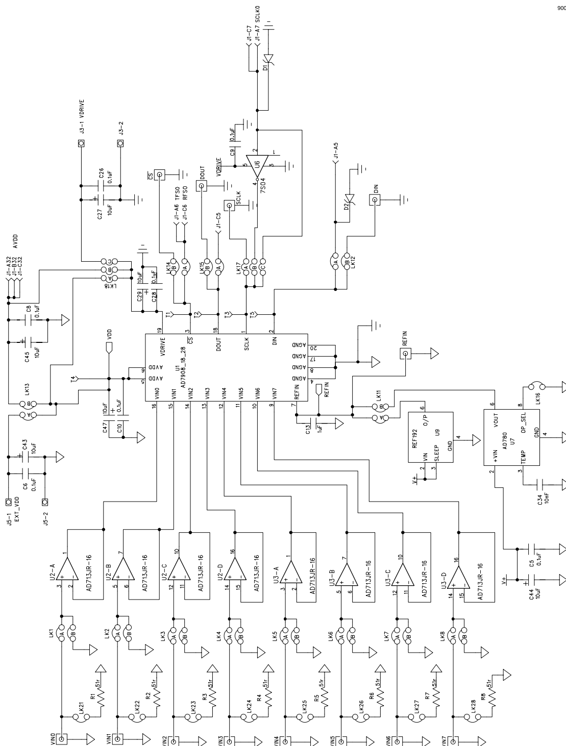
Figure 6. Schematic 1
