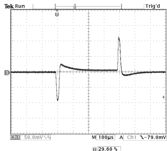
Figure 22. Vin=3V, Vout=1V. Bandwidth is 30kHz
