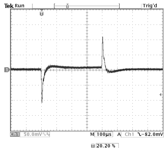
Figure 21. Vin=5V, Vout=2.5V. Bandwidth is 40kHz
