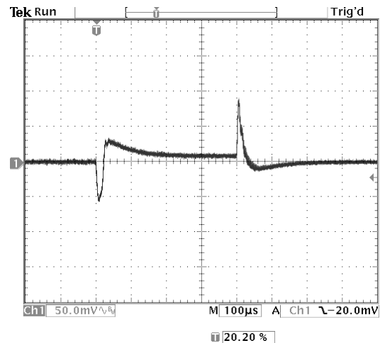
Figure 20. Vin=5V, Vout=1V. Bandwidth is 40kHz
