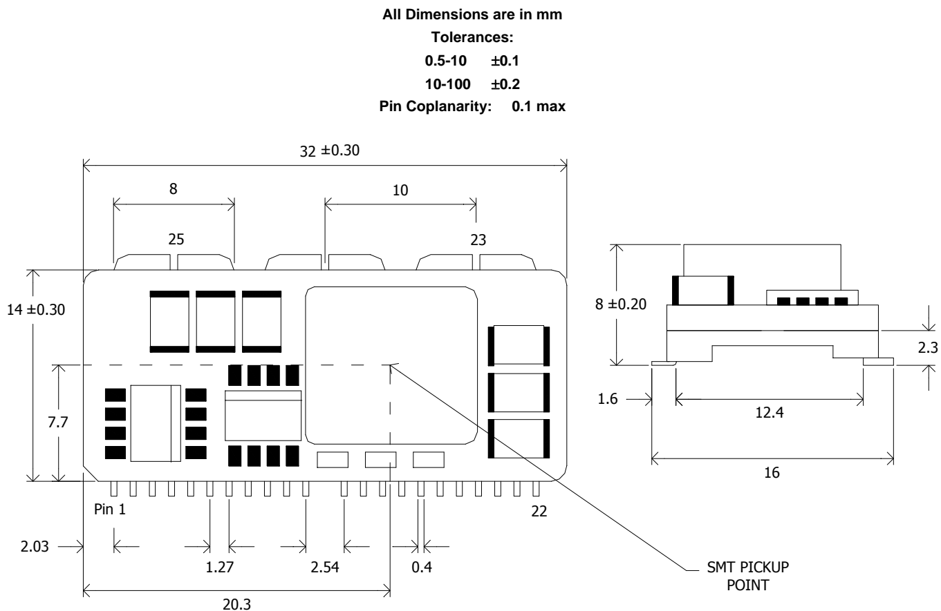
Figure 57. Mechanical Drawing
