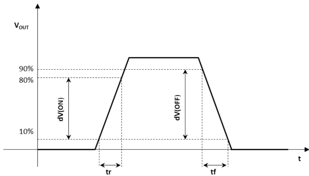
Figure 4. dV/dT
