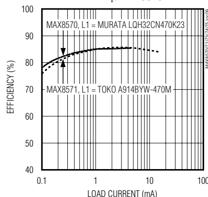
EFFICIENCY vs. LOAD CURRENT WITH 47μH INDUCTOR
