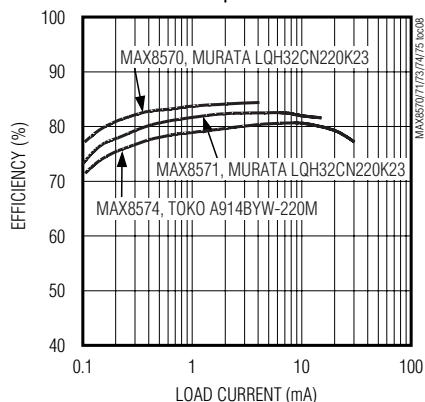
EFFICIENCY vs. LOAD CURRENT WITH 22μH INDUCTOR
