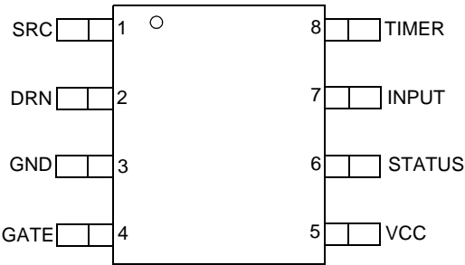
Figure 3. 33198 Pin Connections
