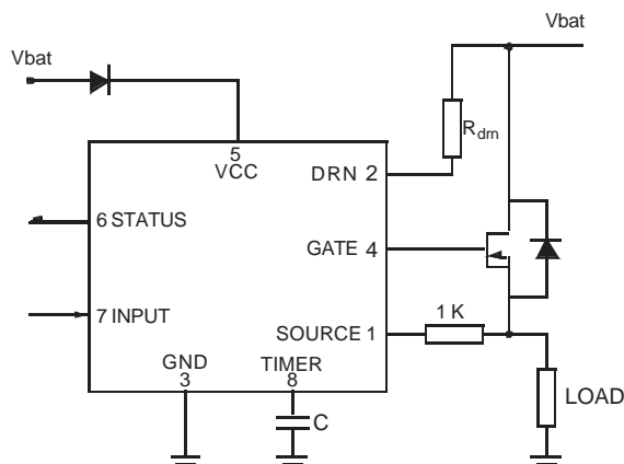
Figure 18. 33198 Reverse Battery
