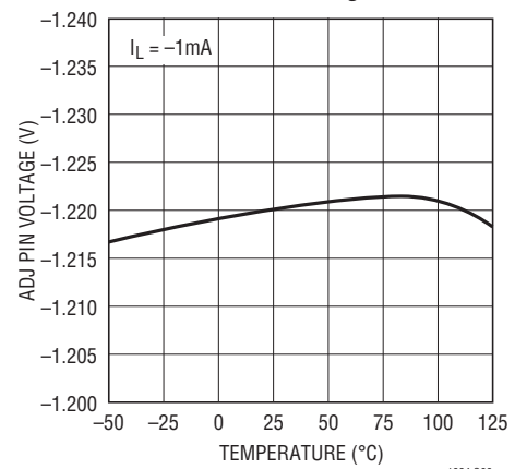
LT1964 ADJ Pin Voltage
