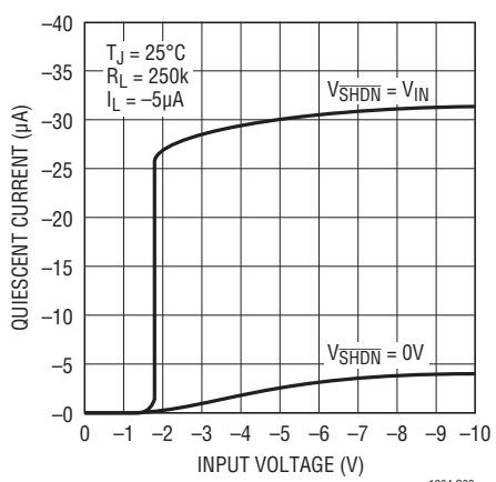
LT1964 Quiescent Current
