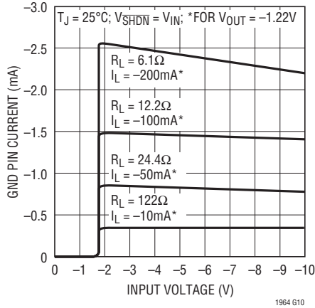
LT1964 GND Pin Current
