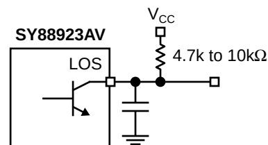
Figure 1. LOS Output with Desired Rise Time
