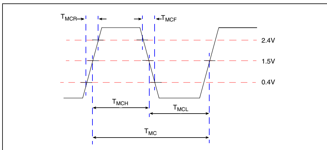
Figure 7. MCLK Waveform
