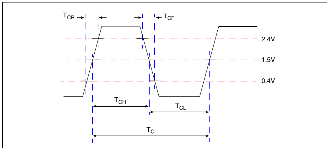
Figure 7. MCLK Waveform
