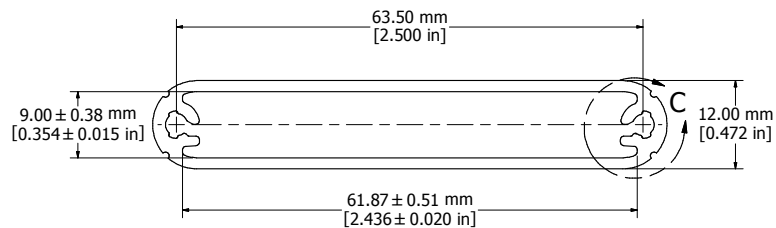
EXTRUSION
