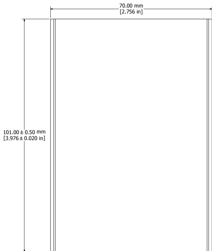
EXTRUSION
