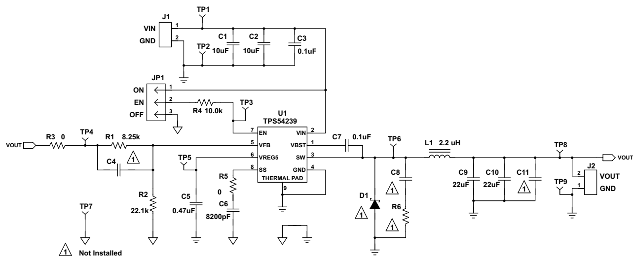
Figure 6-1. TPS54239EVM-056 Schematic Diagram
