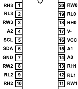
ISL22343 (20 LEAD TSSOP) TOP VIEW
