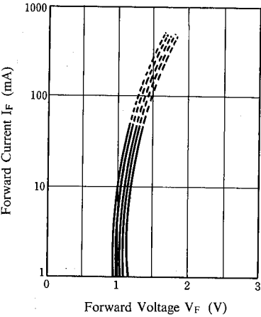
Forward Current vs. Forward Voltage ( T_a=75, 50, 25, 0, -25^{\circ}\text{C} )
