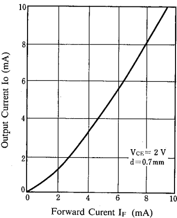
Output Current vs. Forward Current ( T_a=25^{\circ}\text{C} )
