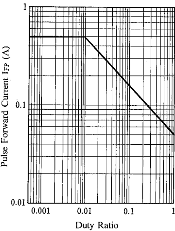
Pulse Forward Current vs. Duty Ratio ( T_a=25^{\circ}\text{C} , t_w=10\mu\text{s} max.)
