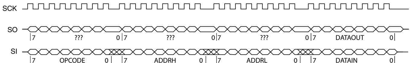
Figure 39-1. ISP Command Sequence
