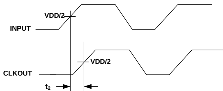
Figure 3. Input-to-Output Skew
