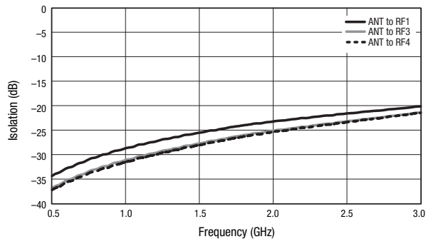
Figure 5. Isolation vs Frequency (ANT to RF2 Insertion Loss State)
