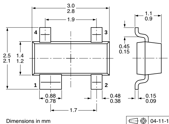
Fig 6. Package outline BAT74 (SOT143B)
