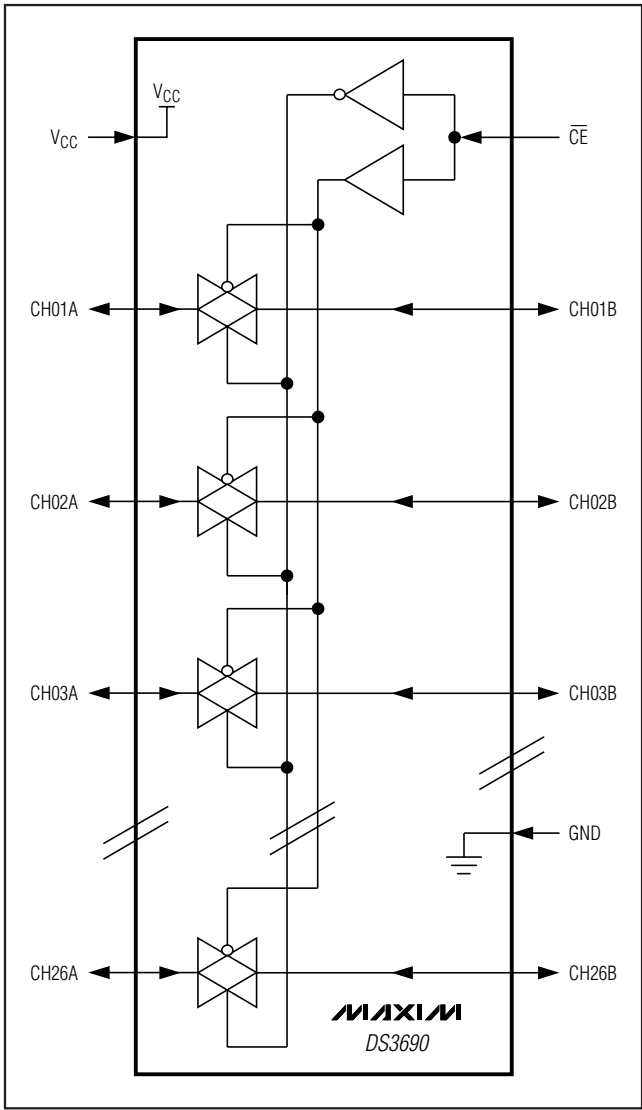
Functional Diagram
