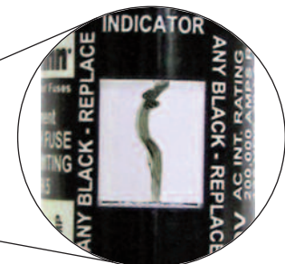
Indicator Shows When Fuse is Blown
