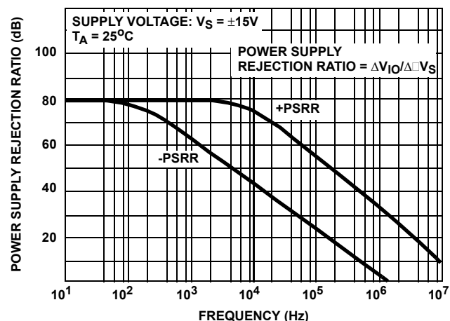
FIGURE 19. POWER SUPPLY REJECTION RATIO vs FREQUENCY
