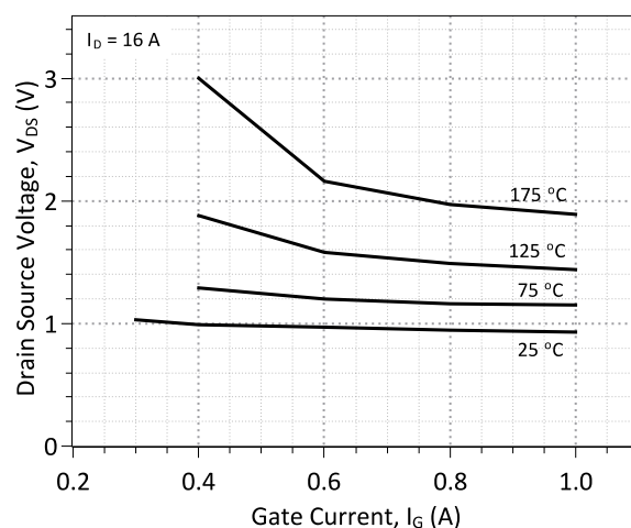
Figure 4: Drain-Source Voltage vs. Gate Current
