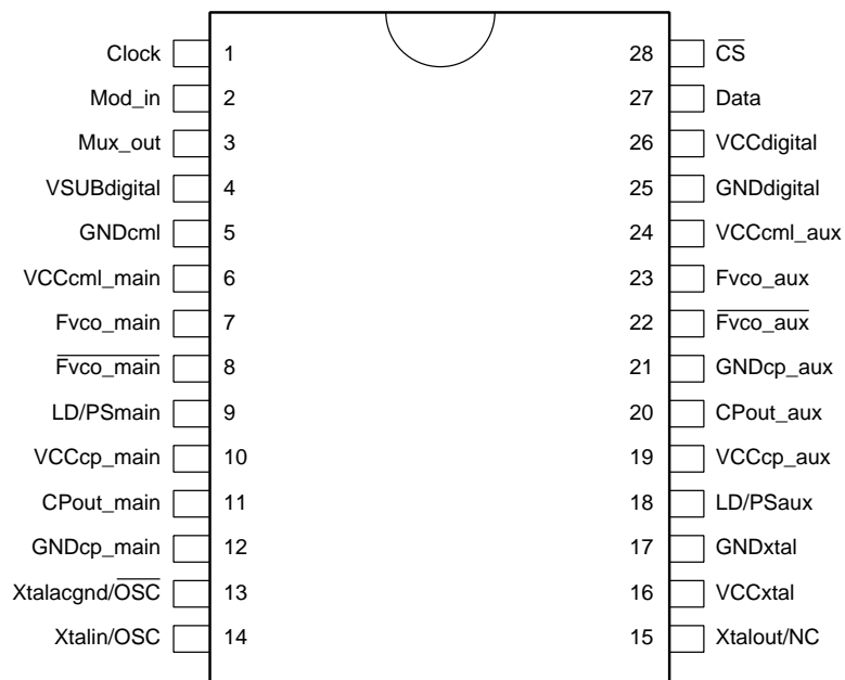
Figure 2. CX72300 Pinout, 28-Pin EP-TSSOP
