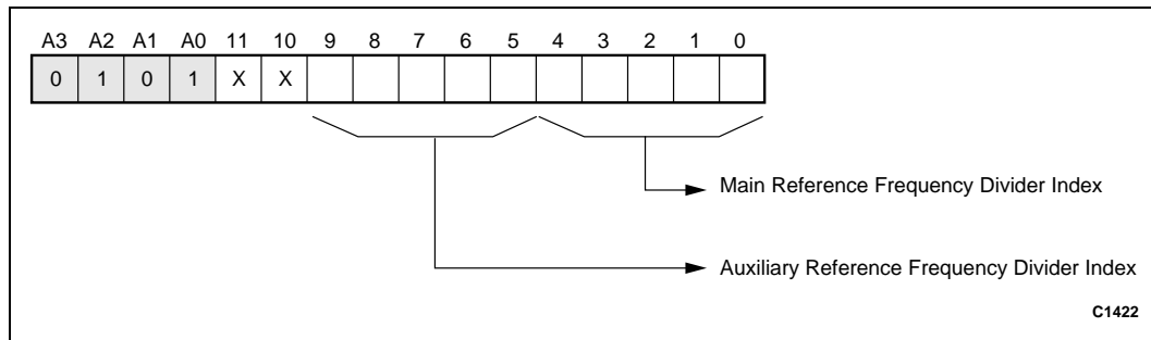
Figure 11. Reference Frequency Dividers Register (Write Only)
