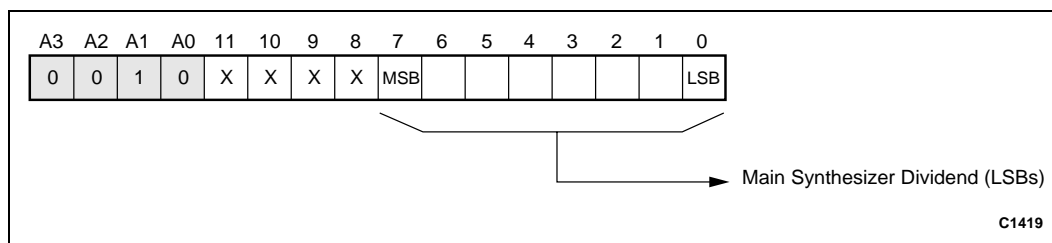
Figure 8. Main Dividend LSB Register (Write Only)
