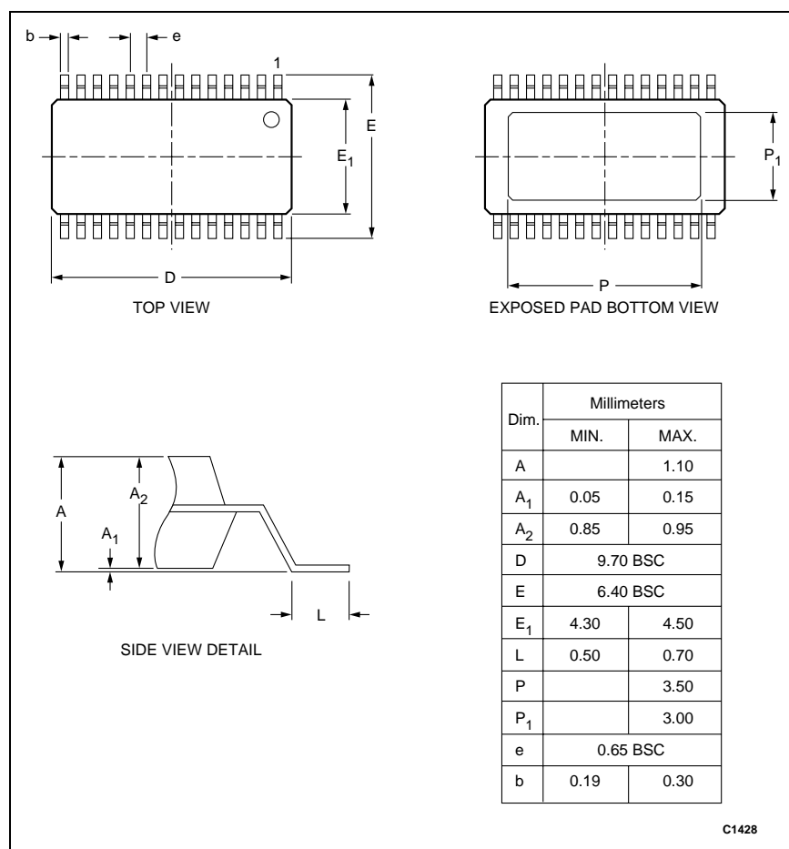
Figure 17. CX72300 28-Pin EP-TSSOP Package Dimension Drawing
