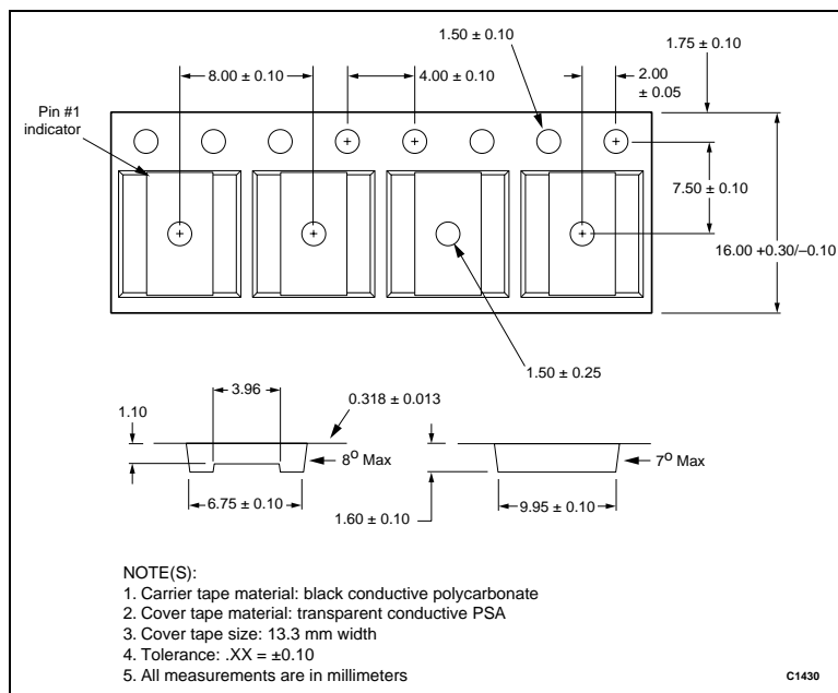
Figure 18. CX72300 Tape and Reel Dimensions
