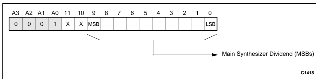
Figure 7. Main Dividend MSB Register (Write Only)
