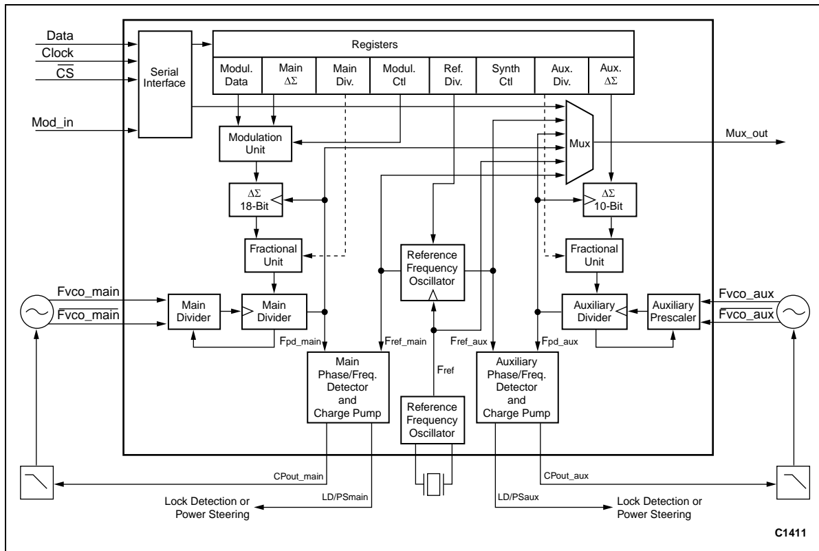
Figure 1. CX72300 Functional Block Diagram
