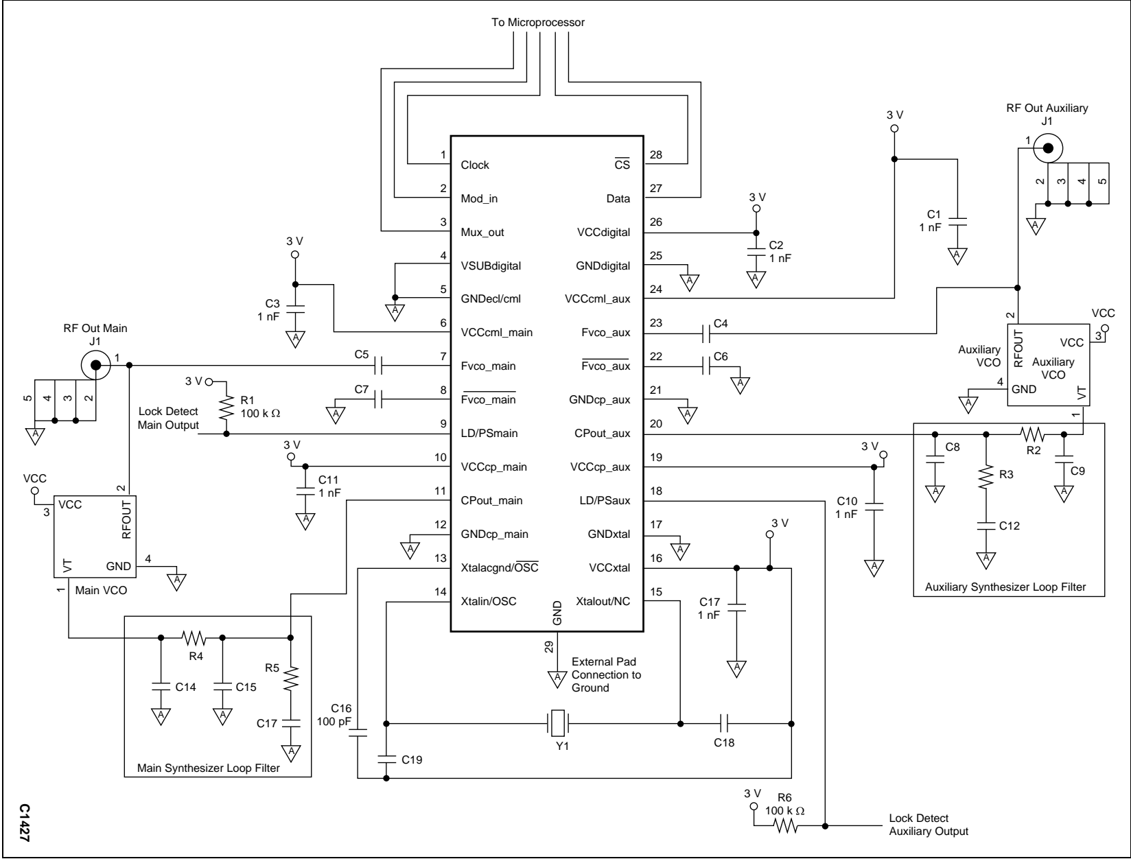
Figure 16. CX72300 Application Schematic
