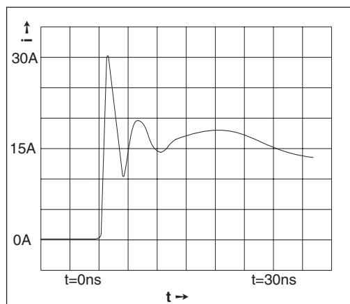
Figure 32. ESD Test Waveform for IEC1000-4-2
