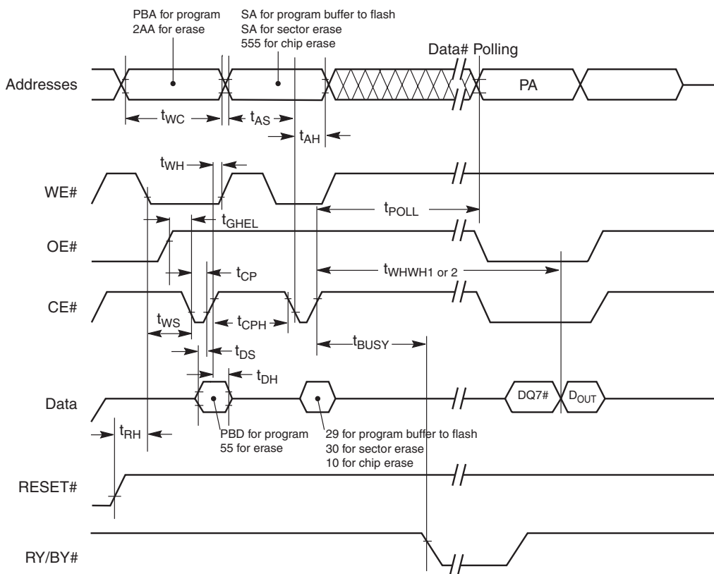
Figure 16.13 Alternate CE# Controlled Write (Erase/Program) Operation Timings
