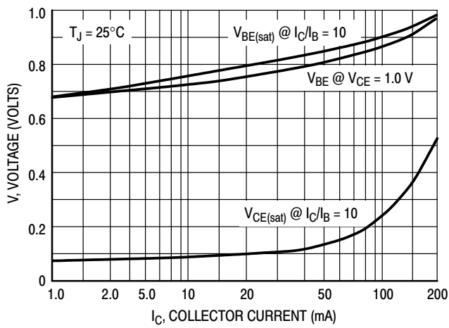
Figure 15. "ON" Voltages
