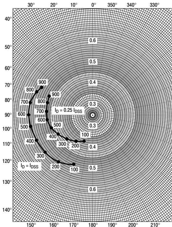
Figure 7. S_{21s}
