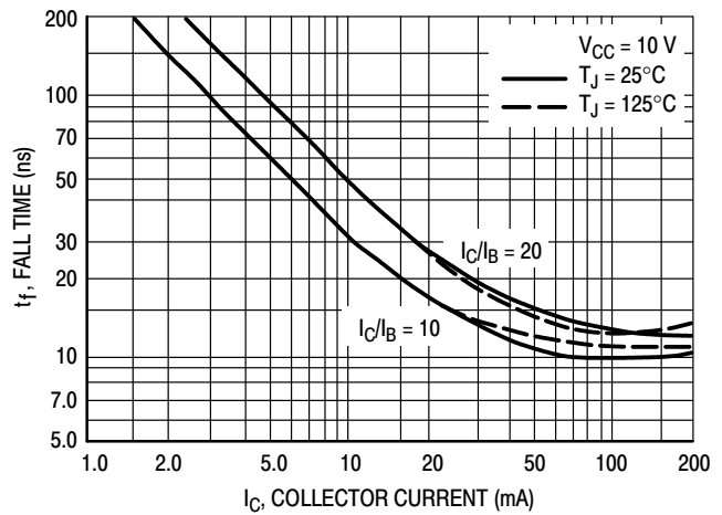
Figure 10. Fall Time
