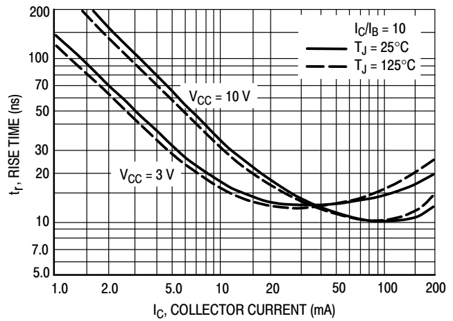
Figure 8. Rise Time
