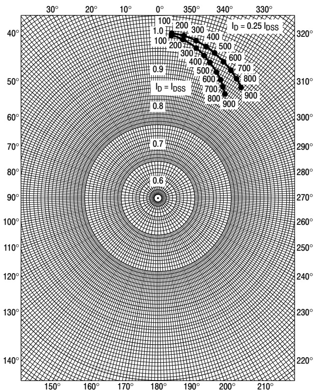
Figure 9. S_{22s}
