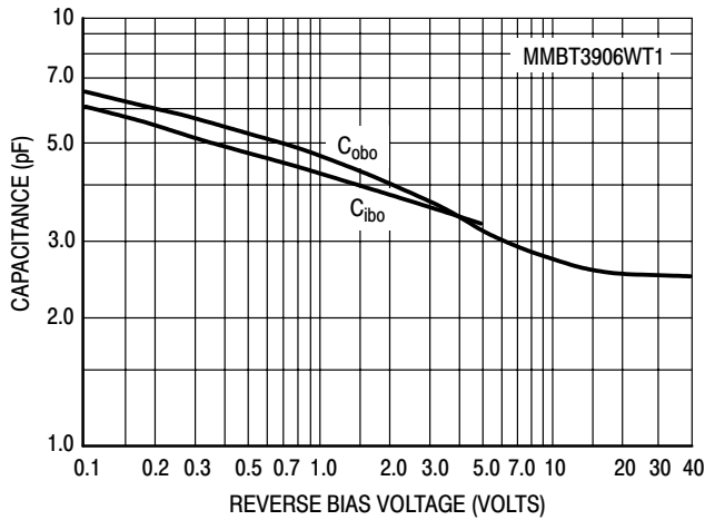
Figure 21. Capacitance
