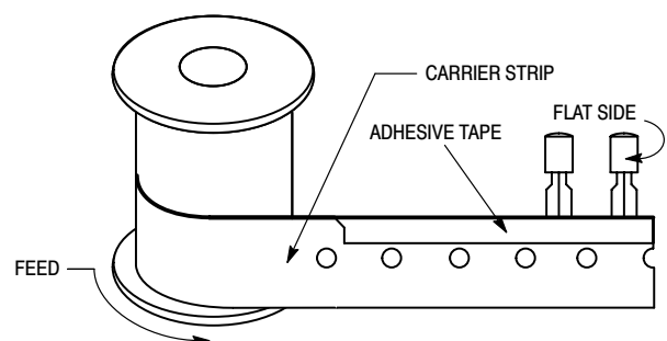
Flat side of transistor and adhesive tape visible.
