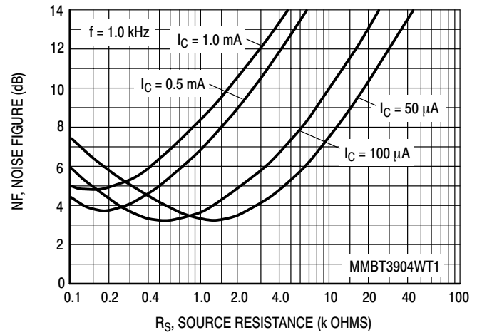
Figure 10. Noise Figure
