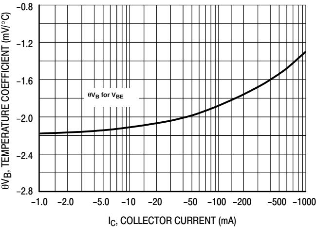
Figure 4. Temperature Coefficient
