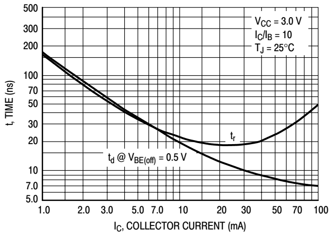
Figure 33. Turn-On Time
