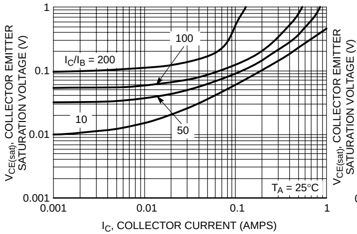
Figure 1. Collector Emitter Saturation Voltage vs. Collector Current
