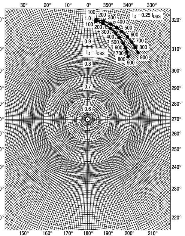
Figure 8. S 22s
