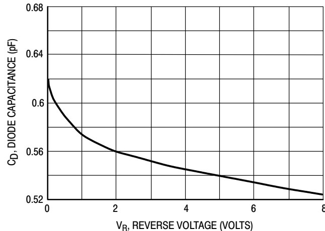
Figure 4. Diode Capacitance
