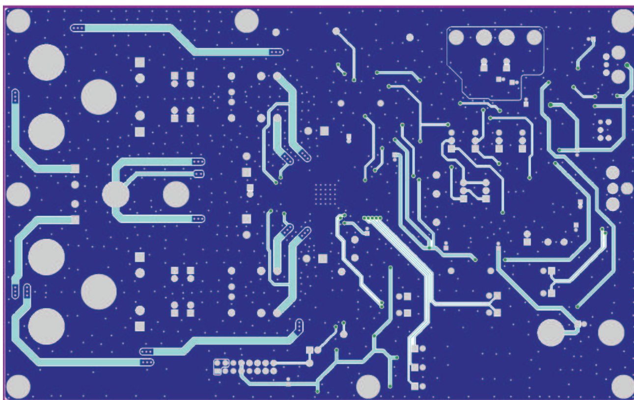
Figure 7. Bottom Layer
