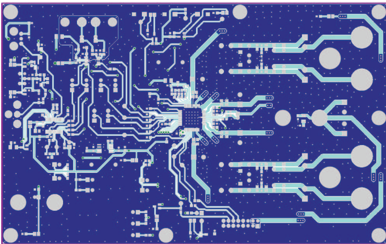
Figure 6. Top Layer
