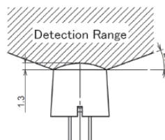
Recommended Hole Drilling Diameter
